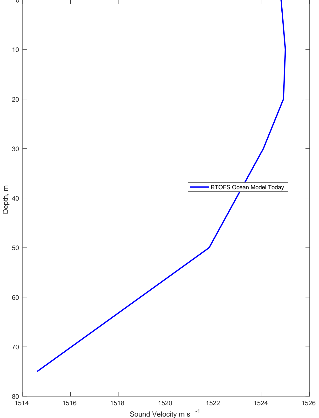
Sound Velocity Profile for BP Senegal YT Nearshore on 02-Feb-2022 00:00:00
